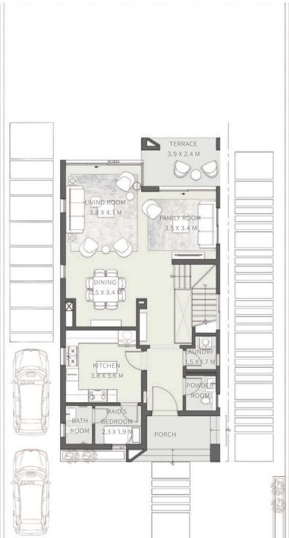
GROUND FLOOR LEVEL
