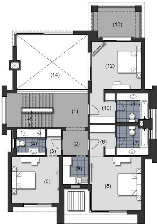
First Floor Total Area = 160.00 m 2
