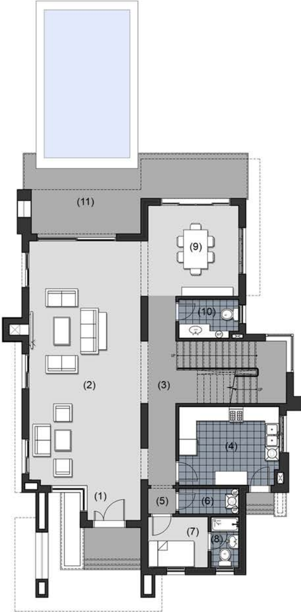
Ground Floor Total Area = 173.00m²
