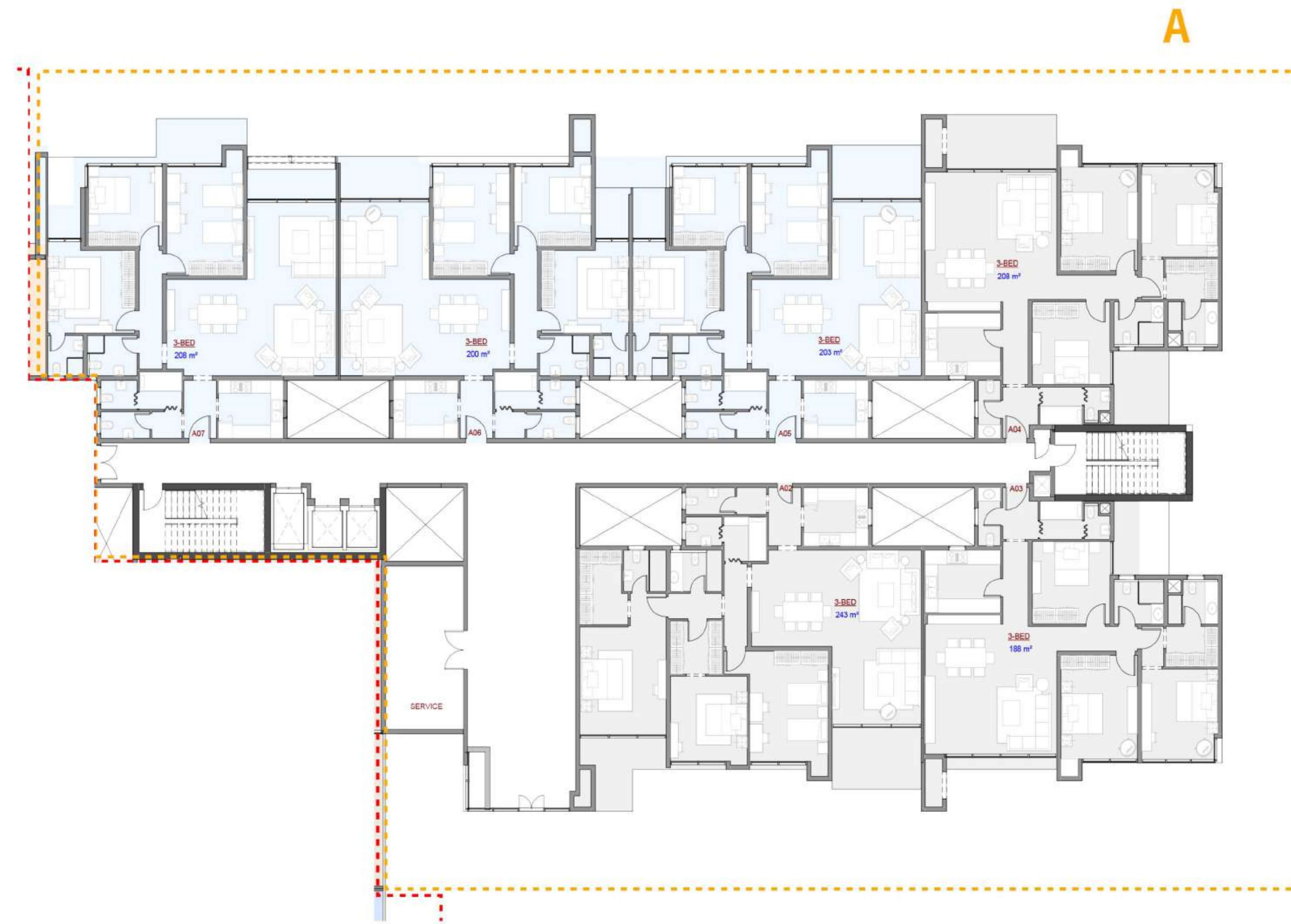
BUILDING TYPE | 02 & 04 GROUND FLOOR
